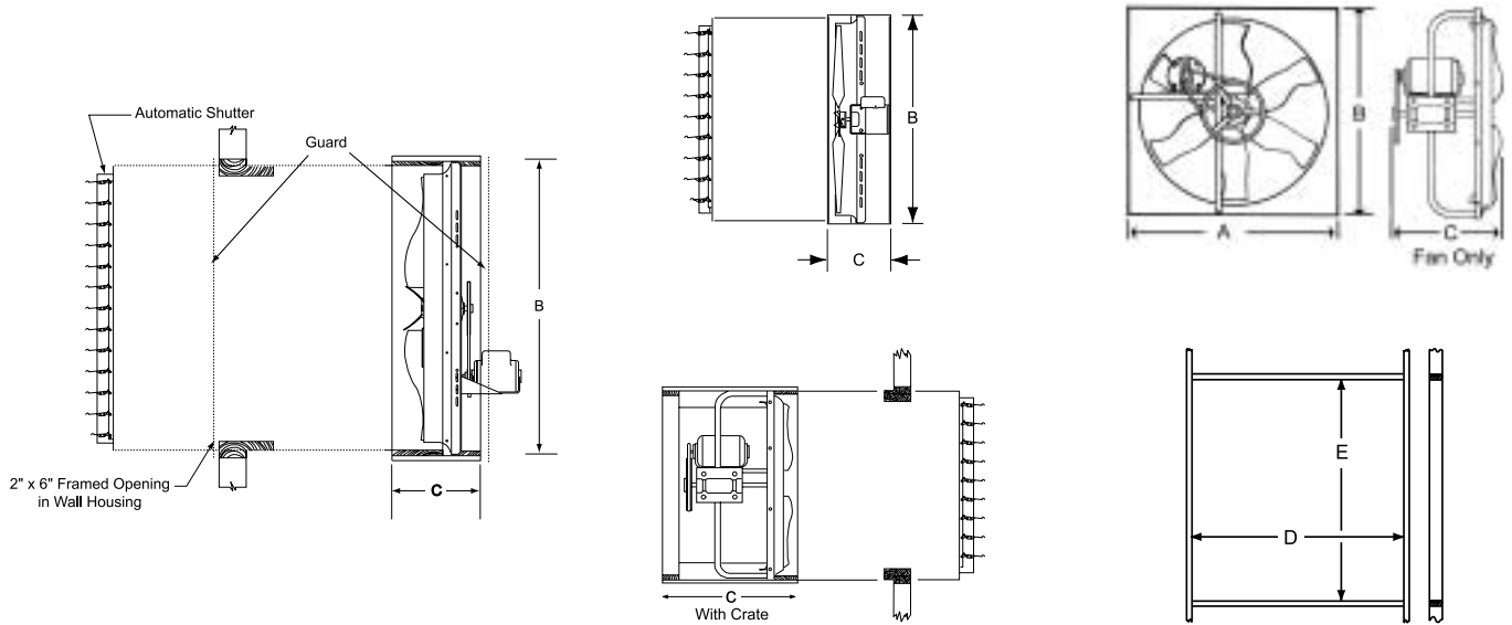
AGD/BDR/ADR Wood Box or Metal Box DC/DCA Fan Only/Crate
